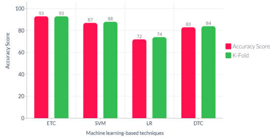
Figure 4. The comparative performance analysis of employed approaches with K-Fold validation
